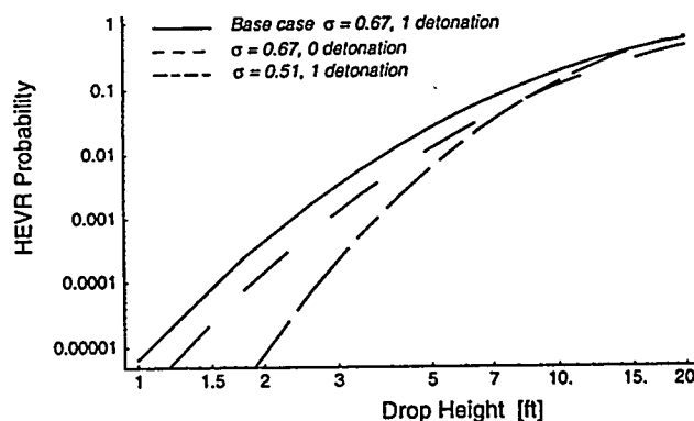
FIG. 1. PROBABILITY OF AN HEVR AS A FUNCTION OF DROP HEIGHT ON NIS FLOORING. CURVES ARE BASED UPON 95% CONFIDENCE LEVEL FOR CERTIFICATION TEST, p_p = 0.05 AND USE AN AVERAGE \mu DERIVED FROM THE TWO DROP TEST PROCEDURES.
